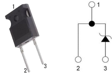
TO-247-2
