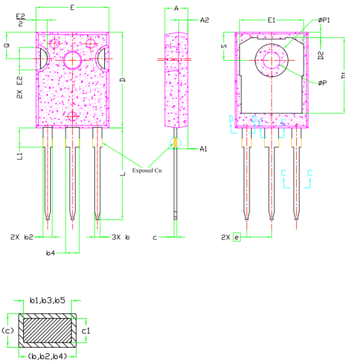
Section C-C, D-D, E-E
